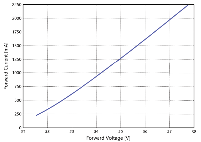
Figure 4f. Typical forward current vs. forward voltage for L2C6-xxxxxL10A1500 at T_j=85^\circ\text{C} .
