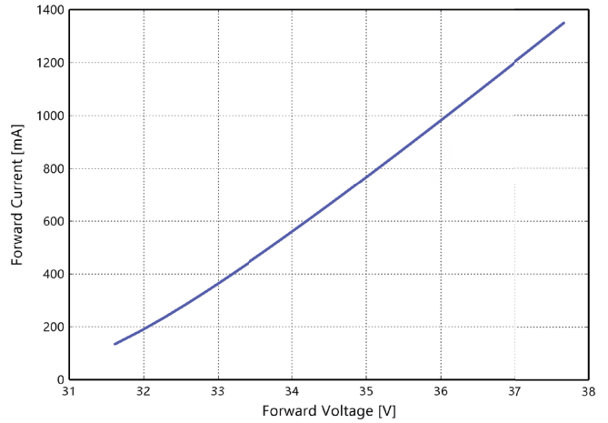
Figure 4d. Typical forward current vs. forward voltage for L2C6-xxxxxL06A1300 at T_j=85^\circ\text{C} .
