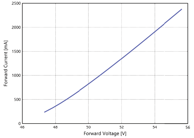
Figure 4j. Typical forward current vs. forward voltage for L2C6-xxxxxR12A2200 at T_j=85^\circ\text{C} .
