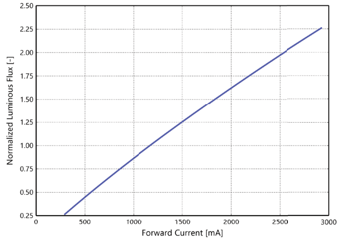
Figure 3h. Typical normalized light output vs. forward current for L2C6-xxxxxL13A2200 at T_j=85^\circ\text{C} .
