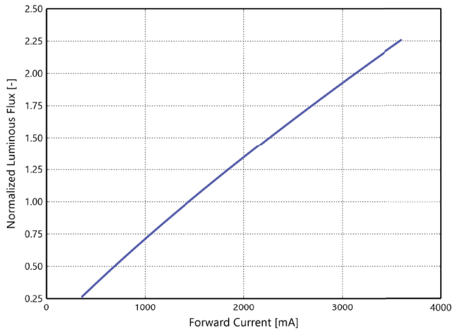
Figure 3i. Typical normalized light output vs. forward current for L2C6-xxxxxL16A2200 at T_j=85^\circ\text{C} .
