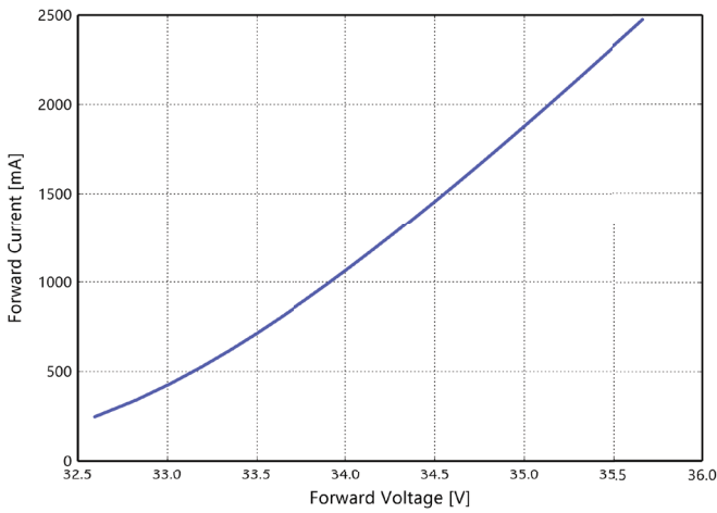
Figure 4g. Typical forward current vs. forward voltage for L2C6-xxxxxL11A2200 at T_j=85^\circ\text{C} .
