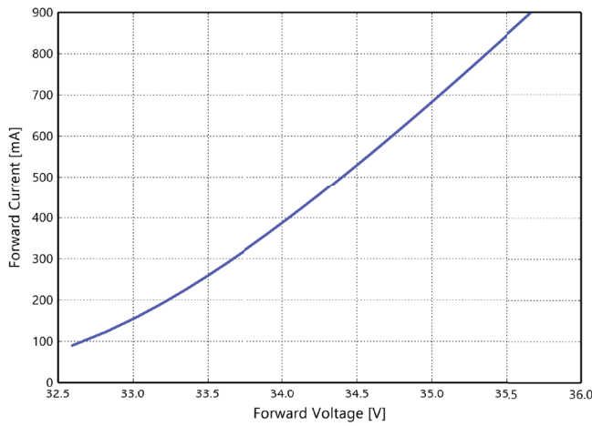
Figure 4c. Typical forward current vs. forward voltage for L2C6-xxxxxL04A0900 at T_j=85^\circ\text{C} .
