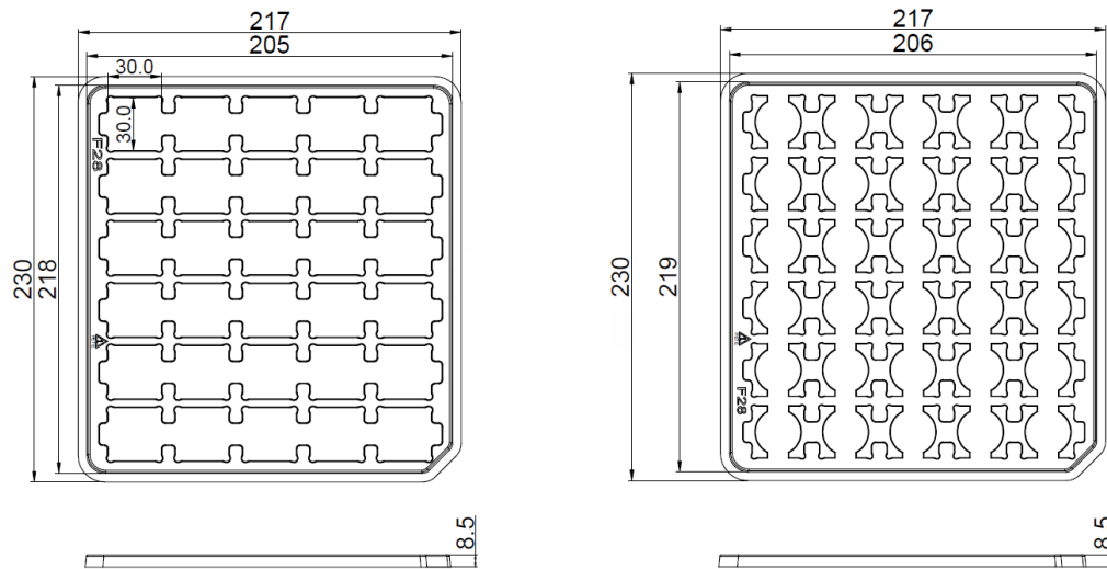
Figure 9c. Tray dimensions for L2C6-xxxxxL06x1300, L2C6-xxxxxL08x1500, L2C6-xxxxxL10x1500.
