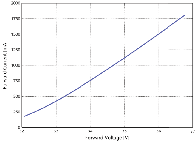
Figure 4e. Typical forward current vs. forward voltage for L2C6-xxxxxL08A1500 at T_j=85^\circ\text{C} .
