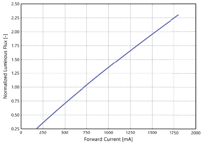
Figure 3e. Typical normalized light output vs. forward current for L2C6-xxxxxL08A1500 at T_j=85^\circ\text{C} .
