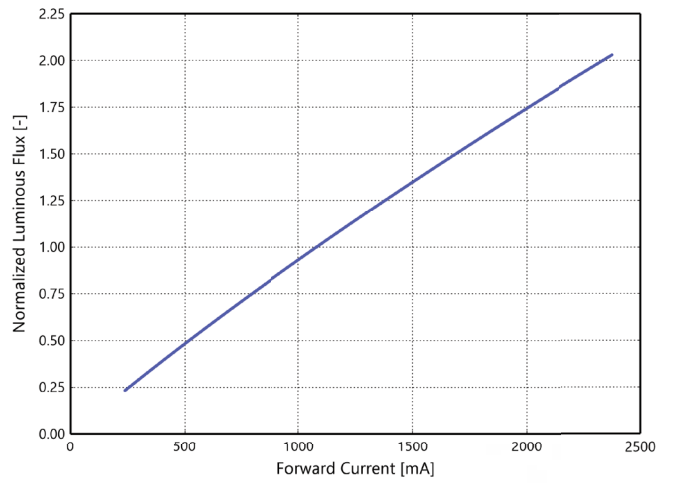
Figure 3j. Typical normalized light output vs. forward current for L2C6-xxxxxR12A2200 at T_j=85^\circ\text{C} .
