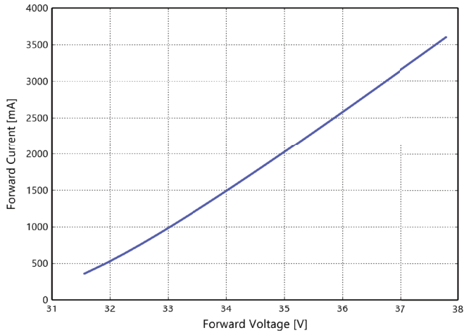
Figure 4i. Typical forward current vs. forward voltage for L2C6-xxxxxL16A2200 at T_j=85^\circ\text{C} .
