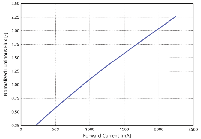
Figure 3f. Typical normalized light output vs. forward current for L2C6-xxxxxL10A1500 at T_j=85^\circ\text{C} .
