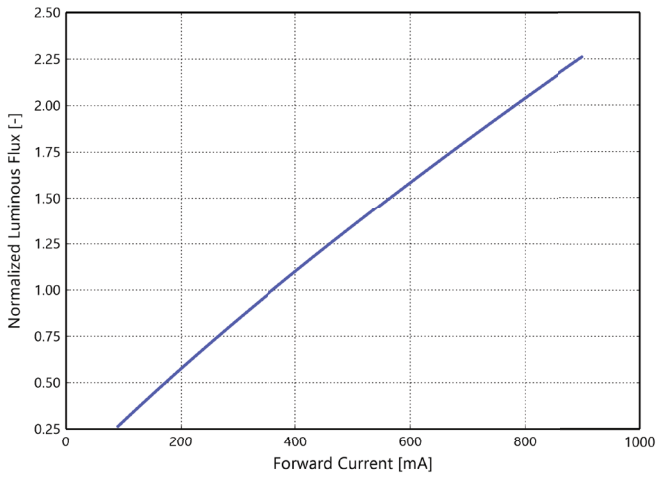
Figure 3c. Typical normalized light output vs. forward current for L2C6-xxxxxL04A0900 at T_j=85^\circ\text{C} .
