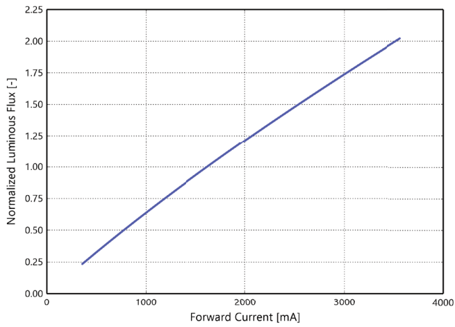
Figure 3k. Typical normalized light output vs. forward current for L2C6-xxxxxR18A2200 at T_j=85^\circ\text{C} .
