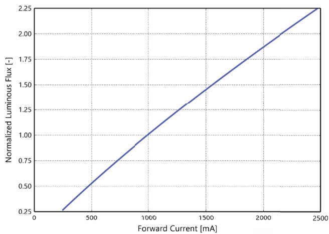
Figure 3g. Typical normalized light output vs. forward current for L2C6-xxxxxL11A2200 at T_j=85^\circ\text{C} .
