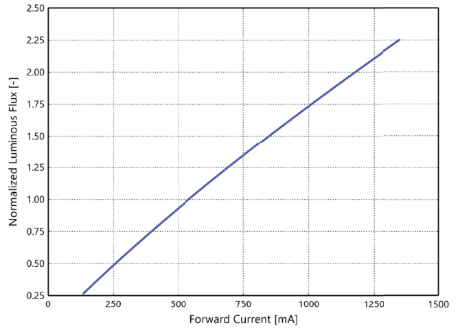
Figure 3d. Typical normalized light output vs. forward current for L2C6-xxxxxL06A1300 at T_j=85^\circ\text{C} .
