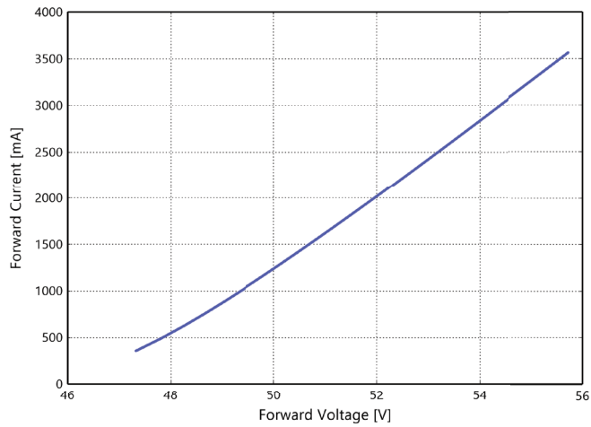
Figure 4k. Typical forward current vs. forward voltage for L2C6-xxxxxR18A2200 at T_j=85^\circ\text{C} .
