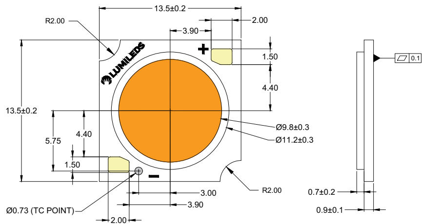
Figure 8b. Mechanical dimensions for L2C6-xxxxxL02x0900 and L2C6-xxxxxL04x0900.
