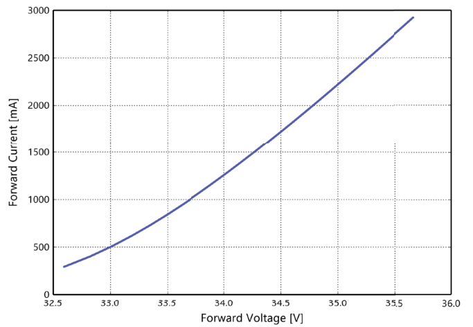
Figure 4h. Typical forward current vs. forward voltage for L2C6-xxxxxL13A2200 at T_j=85^\circ\text{C} .
