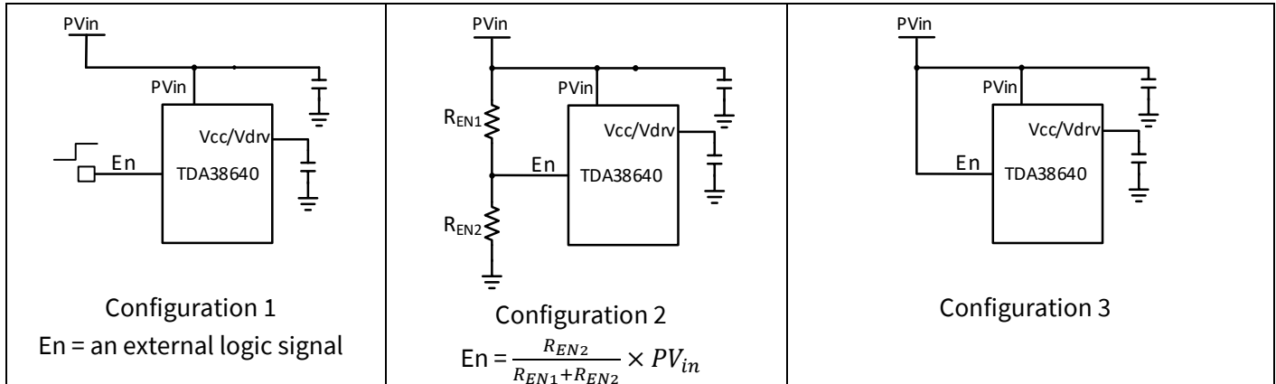
Figure 17 Enable Configurations
