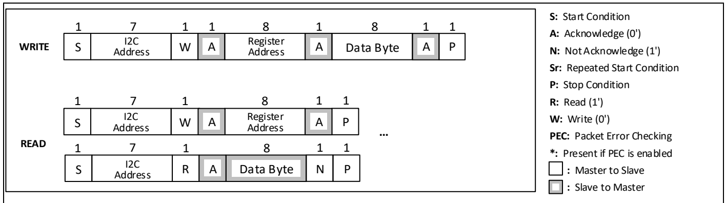
Figure 23 I2C Format
