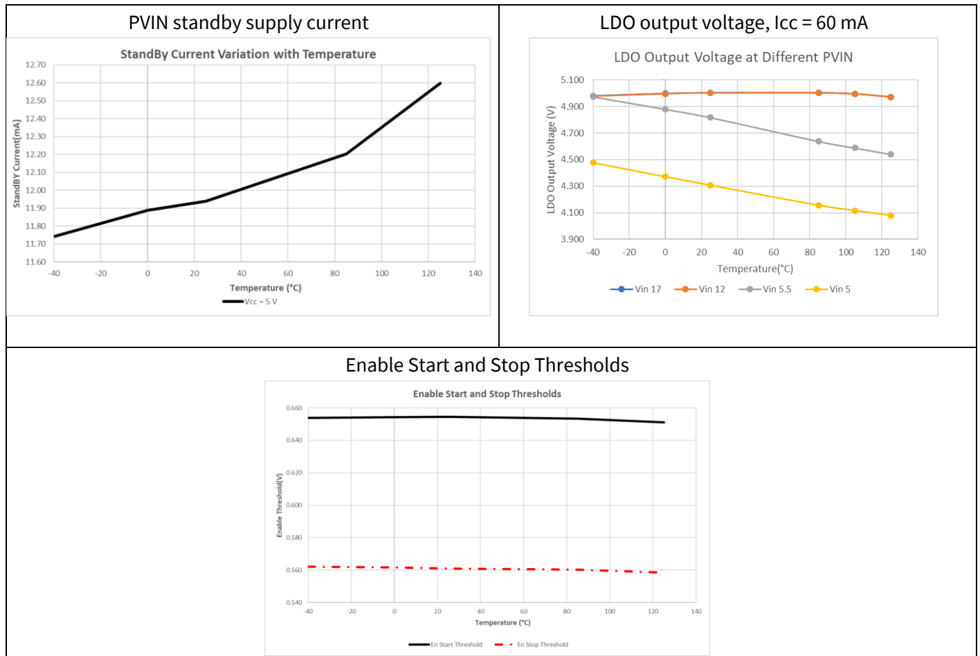
Figure 11 Typical operating characteristics (set 1 of 2)
