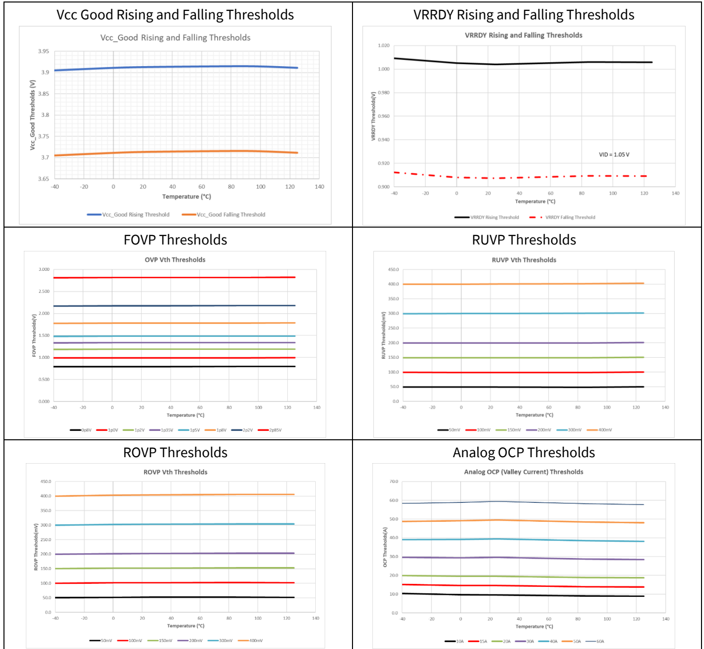
Figure 12 Typical operating characteristics (set 2 of 2)
