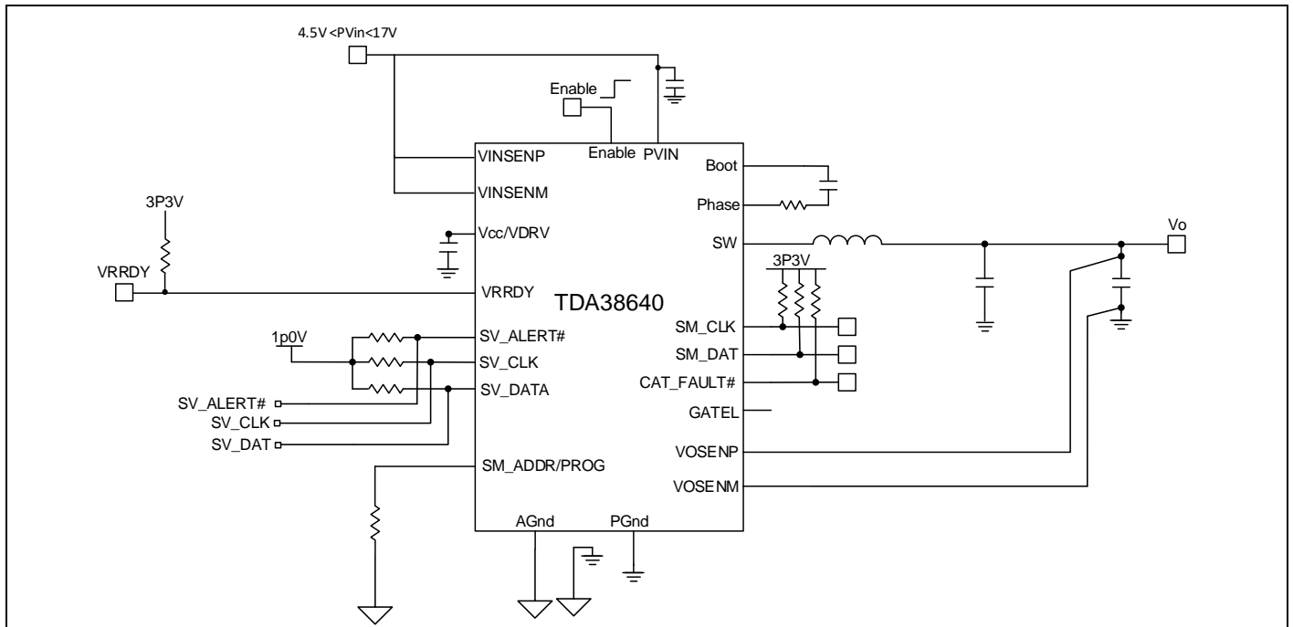
Figure 5 TDA38640 Application Circuit with Input Current Sense Disabled ( 0.25\text{ V} \leq V_{ID} \leq 2.56\text{ V} )
