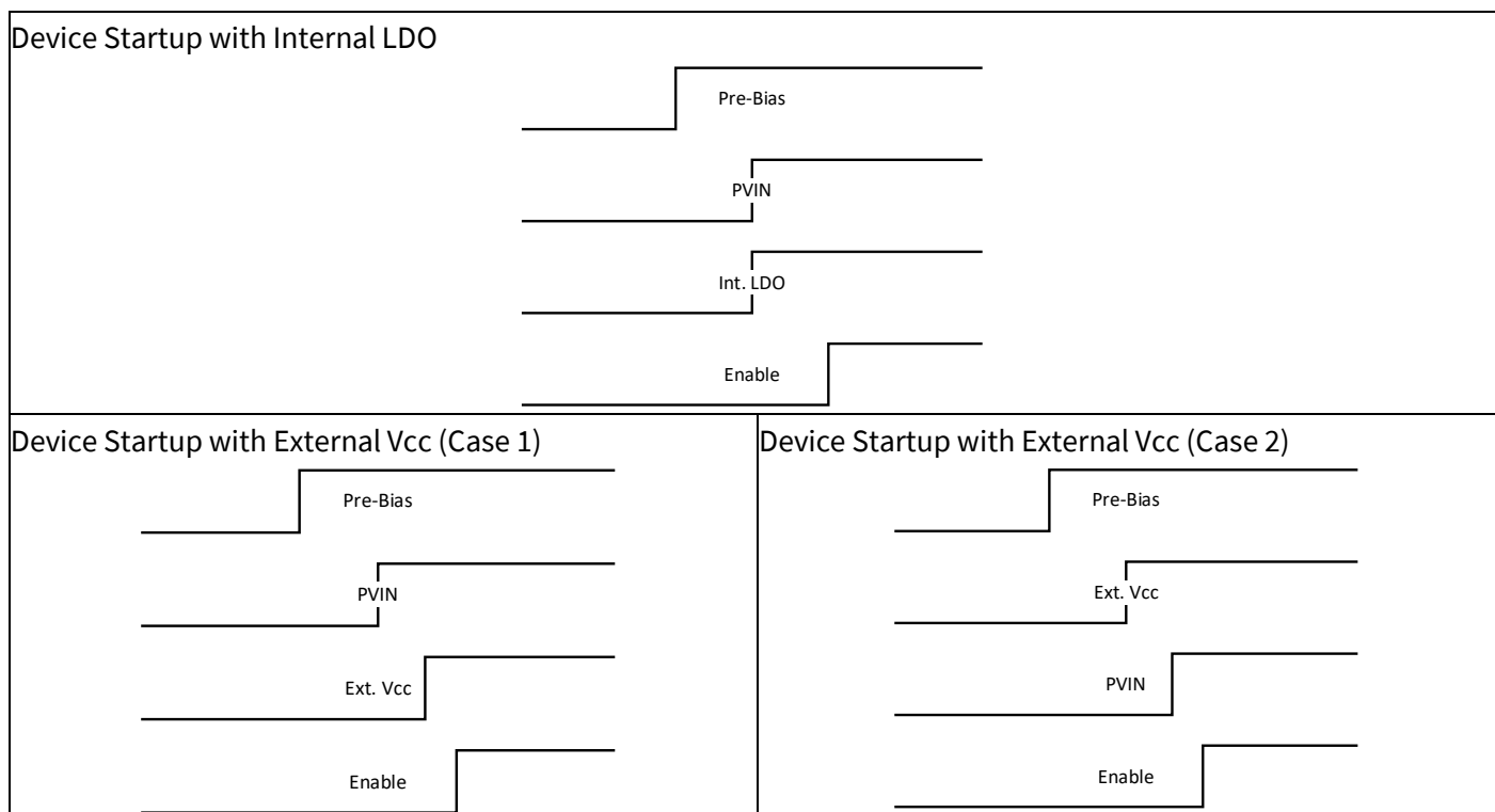
Figure 15 Device power-on sequence with pre-bias.
