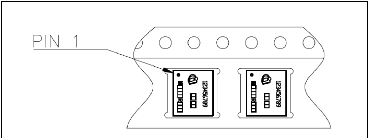
Figure 33 Pin 1 orientation in the Tape & reel
