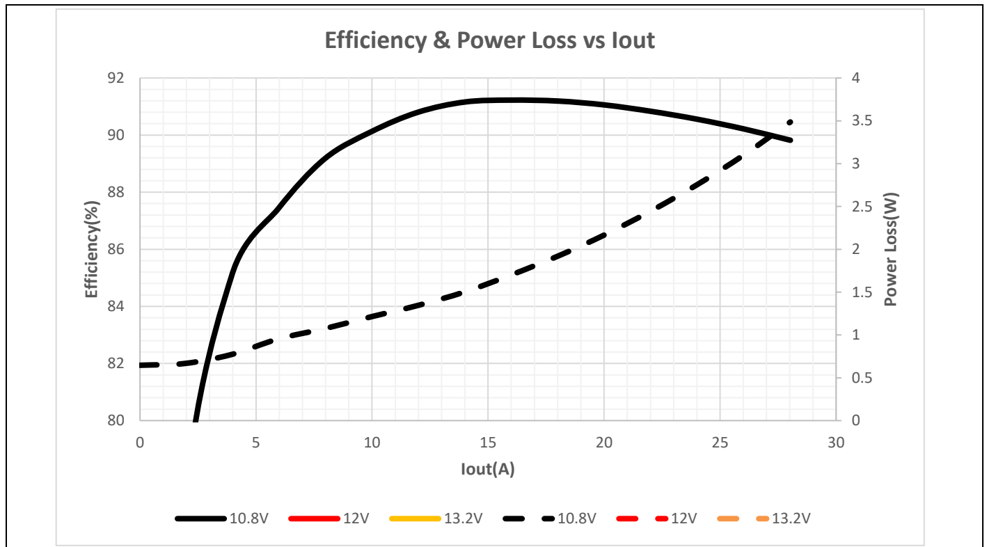
Figure 8 Typical efficiency and power loss curves, P_{V_{in}} = Varying, F_{sw} = 1000 kHz
