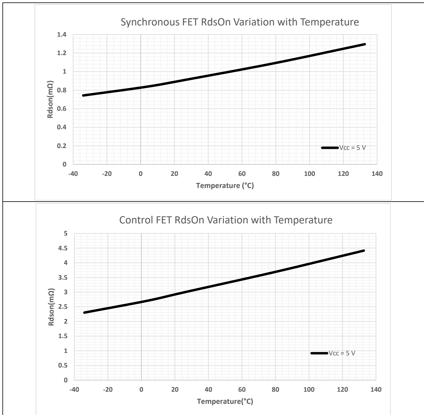
Figure 10 R DS(on) of MOSFETs over Junction Temperature
