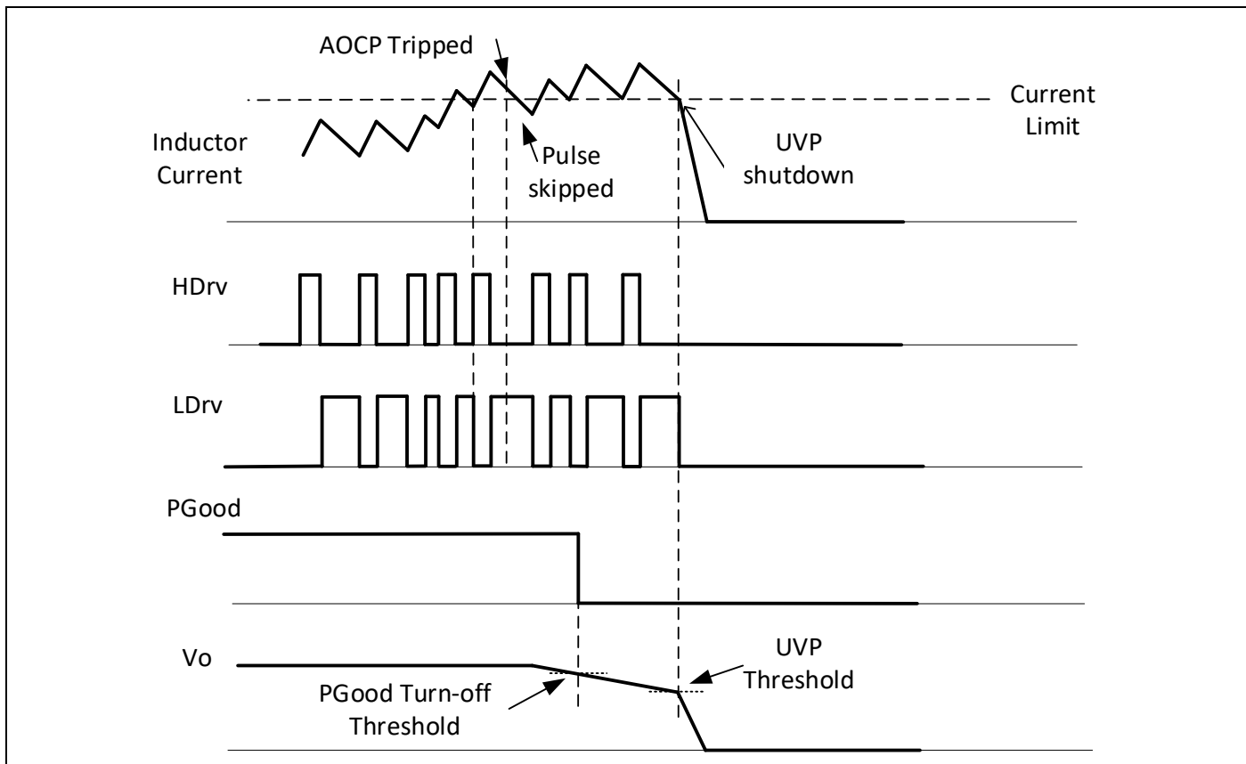
Figure 20 AOCP response timing diagram.
