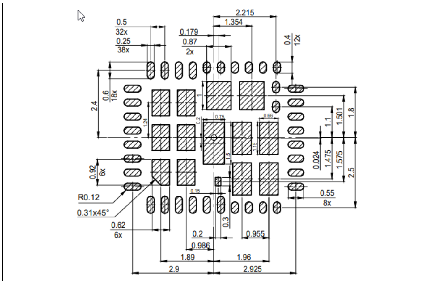
Figure 28 Stencil pad size and spacing (all dimensions in mm)
