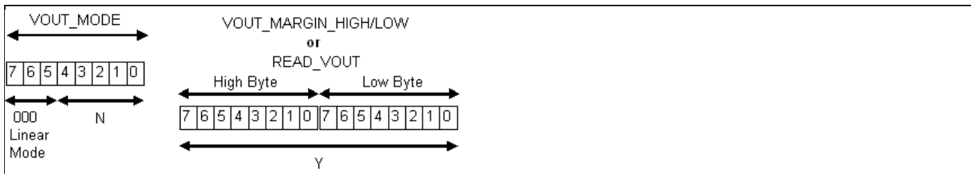
Figure 25 16-BIT Linear Data Format
