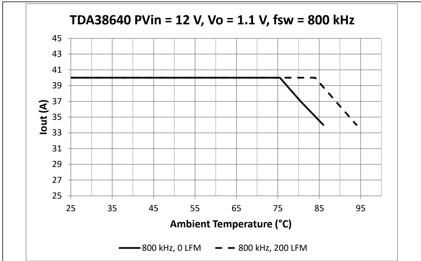
Figure 9 Thermal de-rating curves, P_{Vin} = 12\text{ V} , V_{out}=1.1\text{ V} , f_{sw} = 800\text{ kHz} , VCC = \text{Internal LDO}
