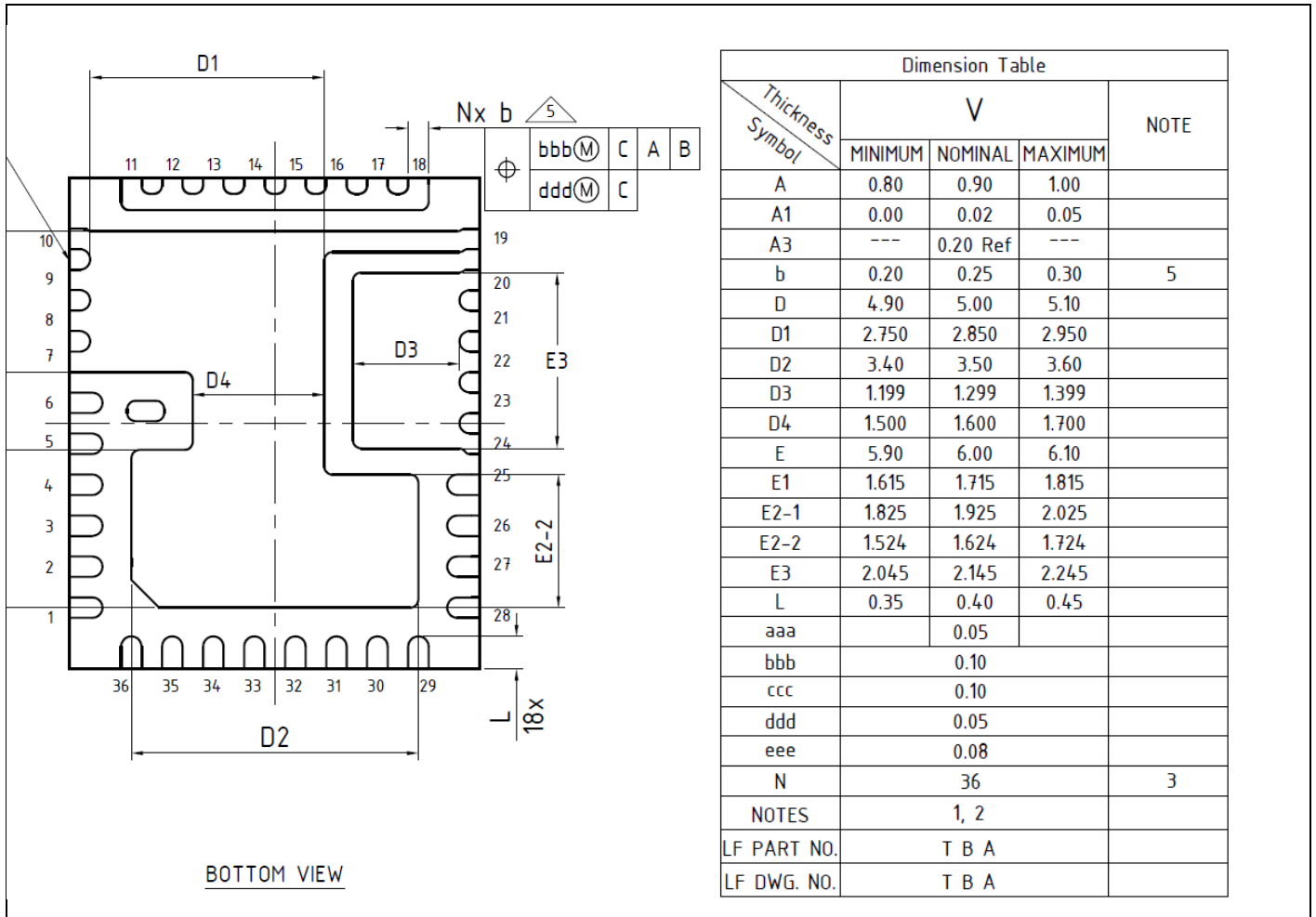
Figure 31 Package Dimensions in mm
