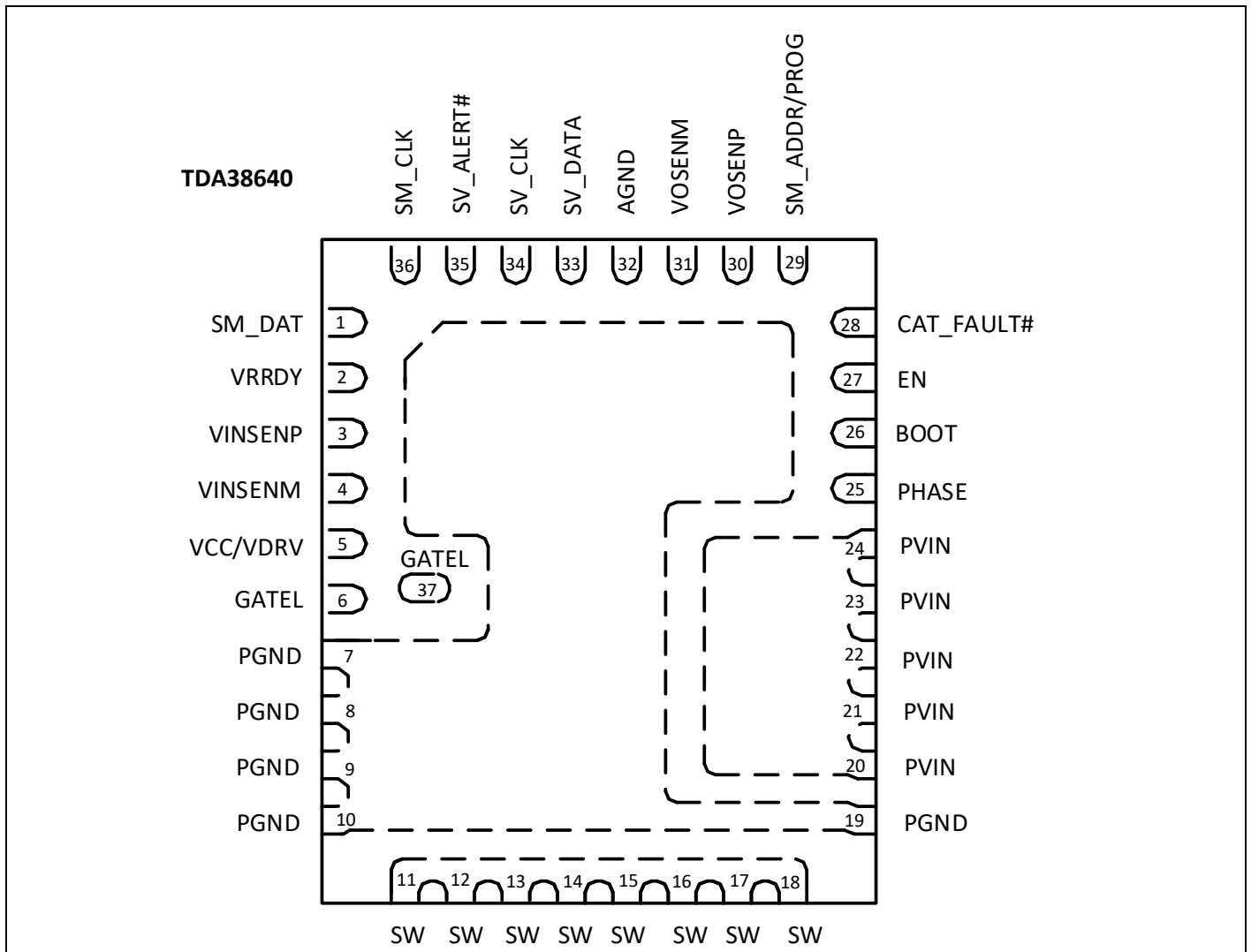
Figure 2 Package Top View
