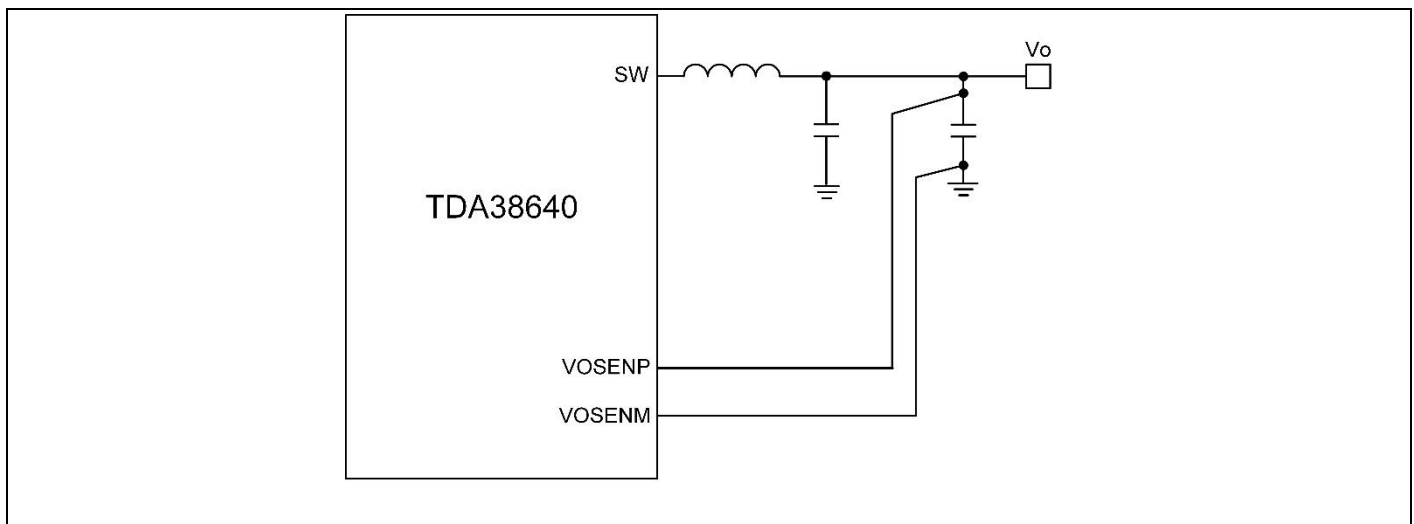
Figure 18 Output voltage sensing connections
