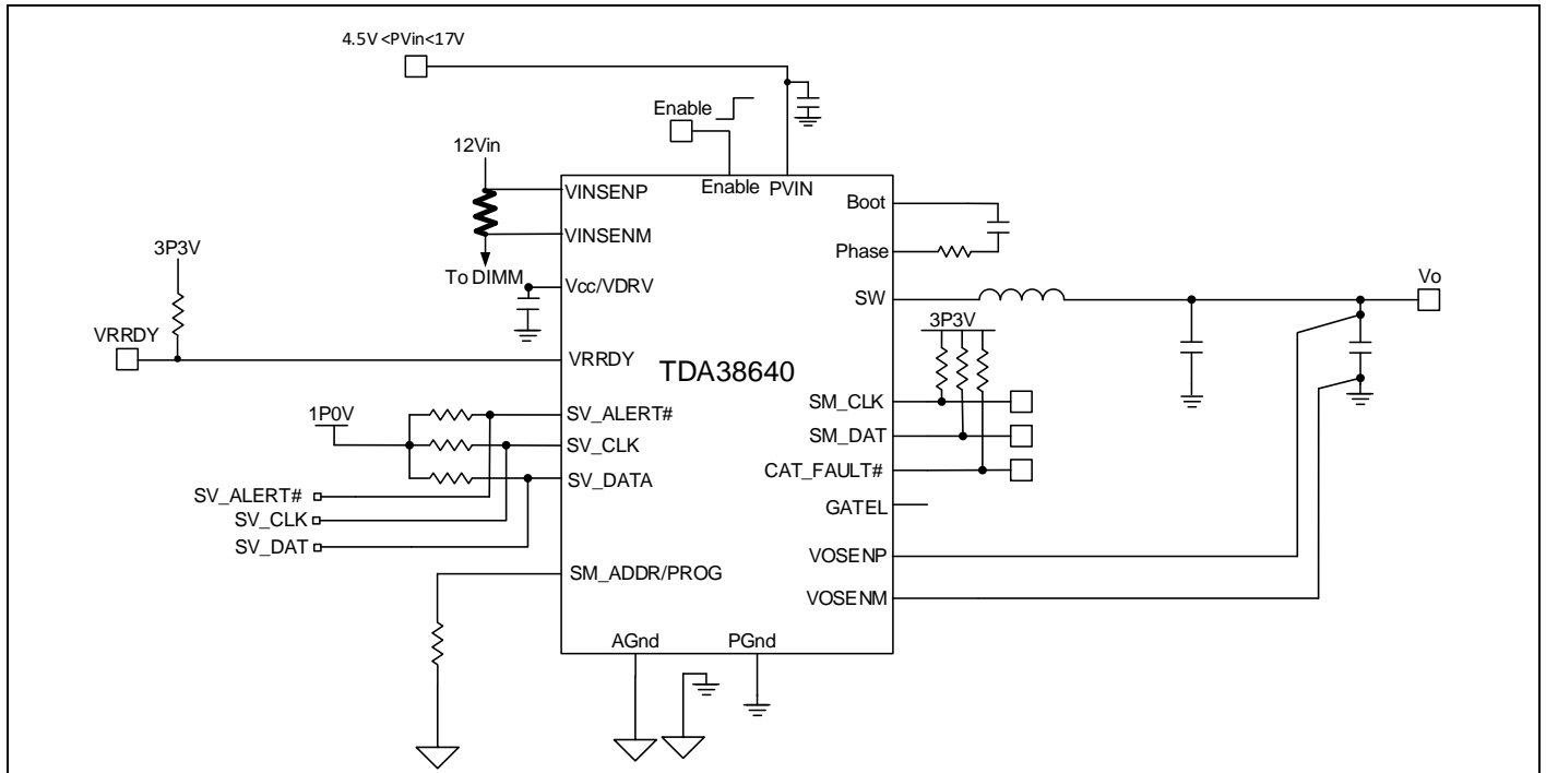
Figure 4 TDA38640 Basic application circuit with Input Current Sense Enabled ( 0.25\text{ V} \leq V_{ID} \leq 2.56\text{ V} )
