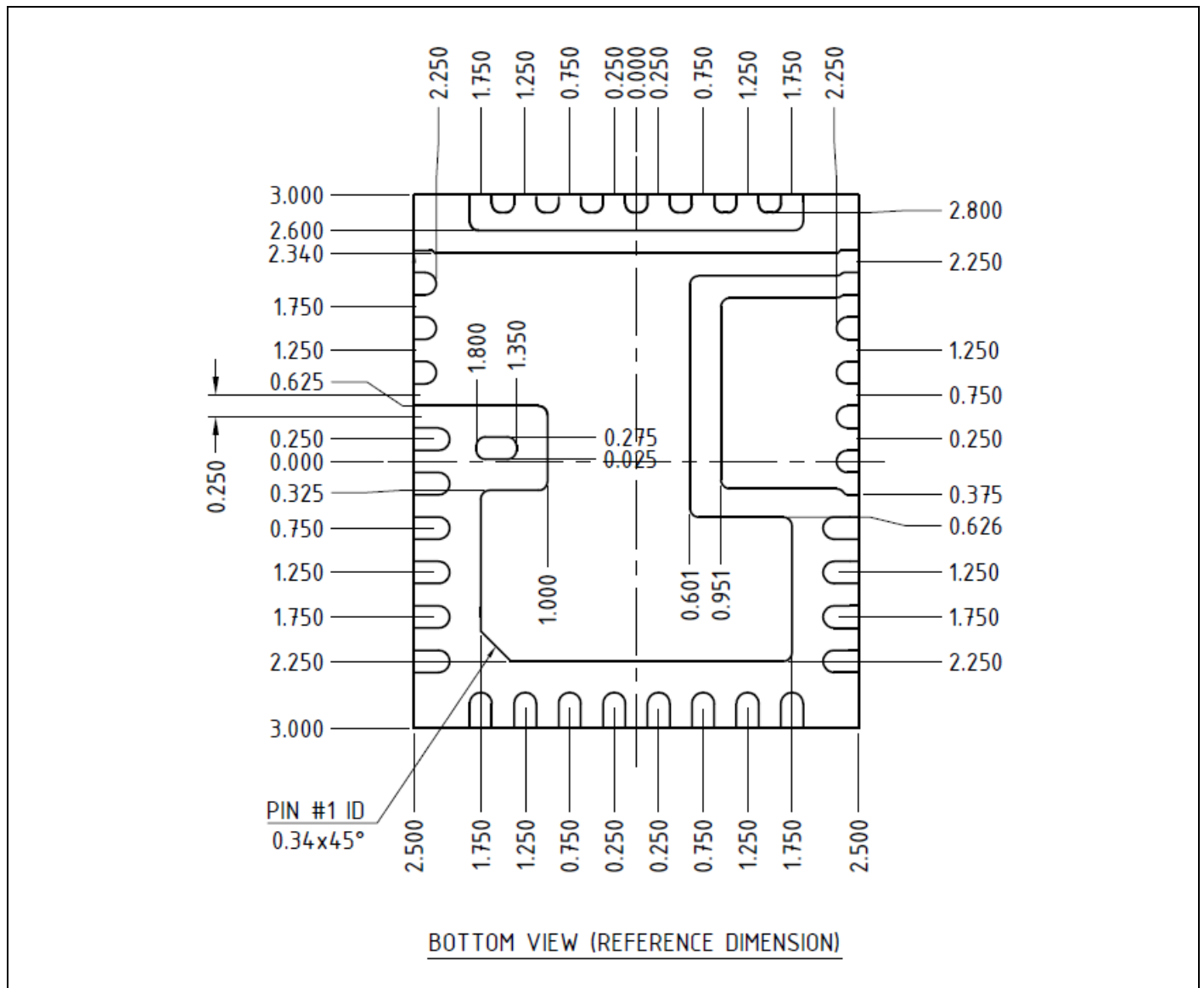
Figure 32 Package Dimensions- Pad Layout
