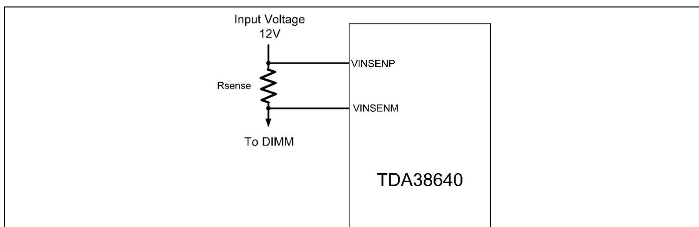
Figure 19 Input current sensing using external shunt
