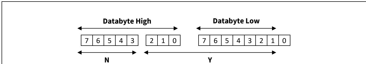
Figure 24 11-Bit Linear Data Format
