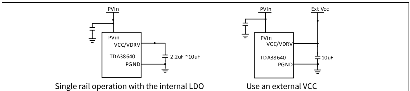
Figure 16 Configuration of using the internal LDO or an external VCC.
