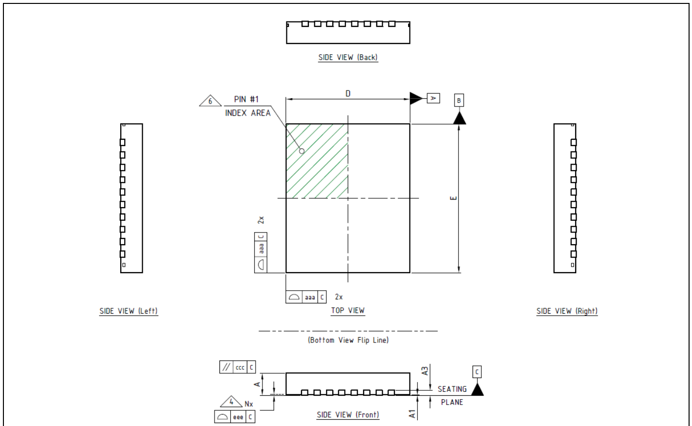
Figure 30 Package view
