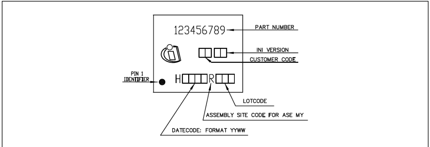
Figure 29 Package Marking
