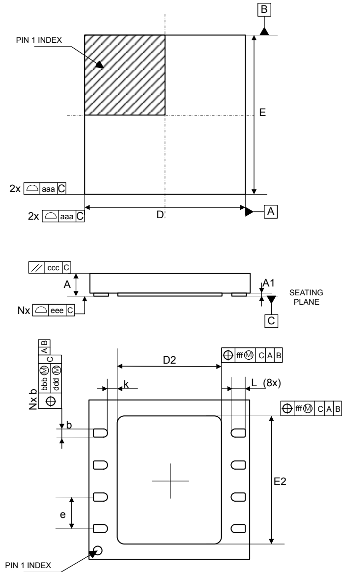
Figure 44. UFDFPN8 - Outline
