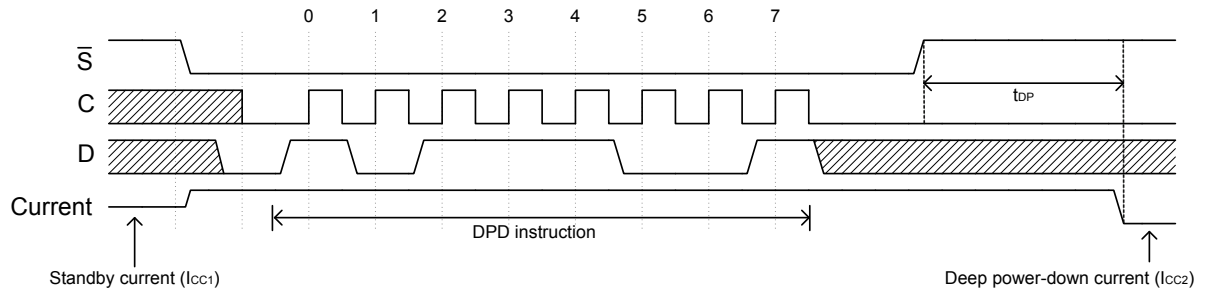
Figure 31. Deep power-down enter
