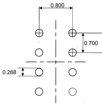
Figure 43. WLCSP8 - Recommended footprint
