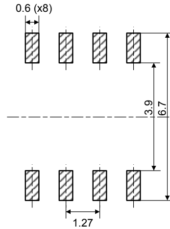
Figure 41. SO8N - Recommended footprint
