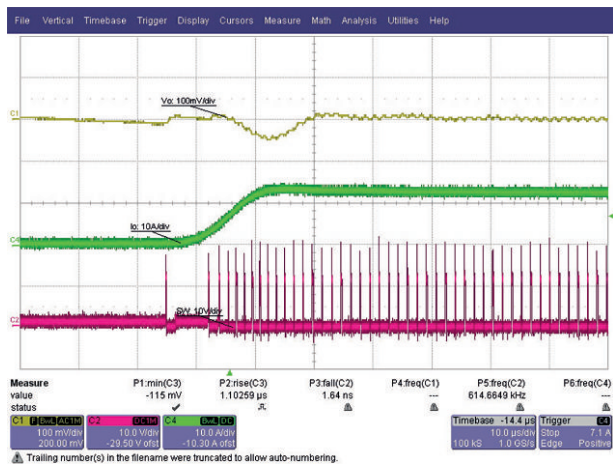
Fig. 28 - Load Step, 0.1 A to 12 A, 1 A/ \mu\text{s} , t = 10\text{ }\mu\text{s}/\text{div} Skip Mode Enabled
