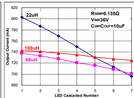
Fig 56. I_{OUT}=740mA
