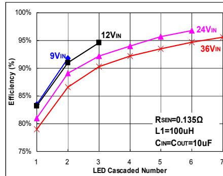
Fig 20. I_{OUT}=740mA
