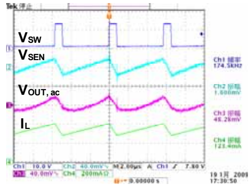
Fig 68. Switching waveform ( 12V_{IN} , 3.6V_{OUT} , R_{SEN}=0.27 )
