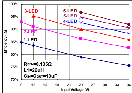
Fig 5. I_{OUT}=740mA
