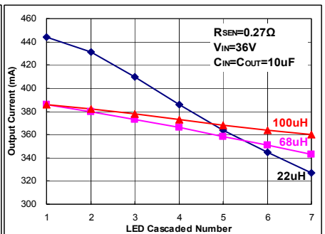
Fig 57. I_{OUT}=370mA
