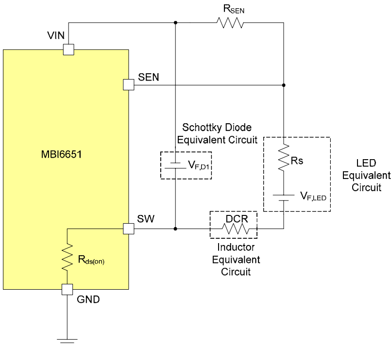
Fig. 78. The equivalent impedance in a MBI6651 application circuit
