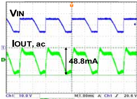
Fig 69. L1=22uH
