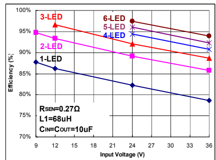
Fig 9. I_{OUT}=370mA
