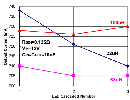
Fig 50. I_{OUT}=740mA
