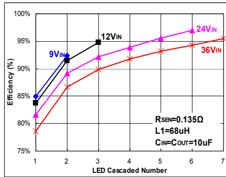
Fig 17. I_{OUT}=740mA
