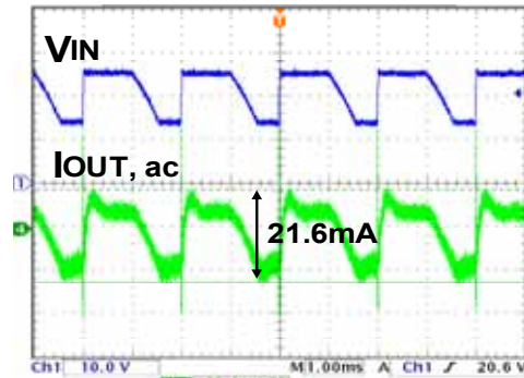
Fig 70. L1=68uH
