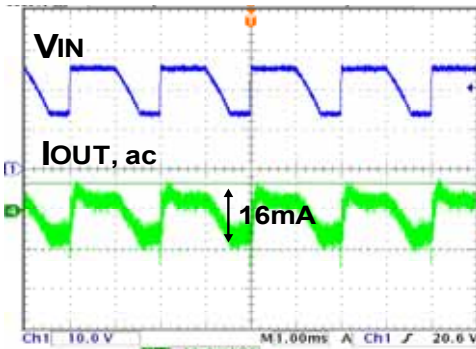
Fig 71. L1=100uH
