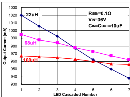
Fig 55. I_{OUT}=1A
