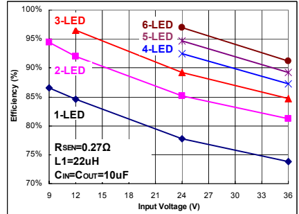
Fig 6. I_{OUT}=370mA
