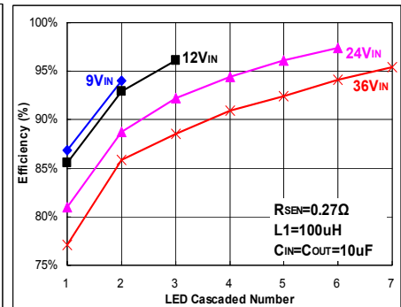
Fig 21. I_{OUT}=370mA
