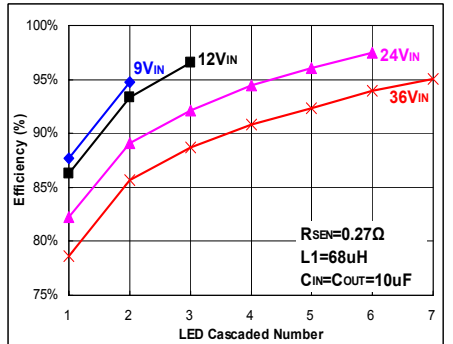
Fig 18. I_{OUT}=370mA
