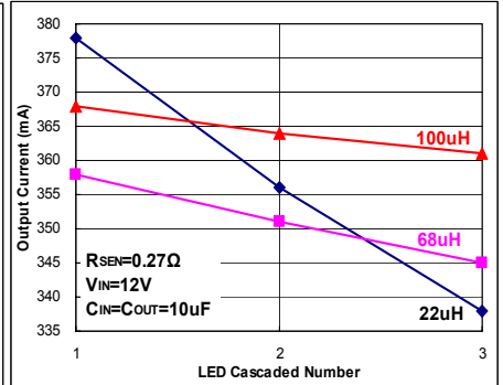
Fig 51. I_{OUT}=370mA
