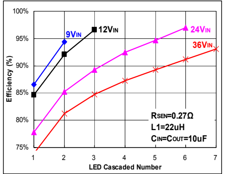
Fig 15. I_{OUT}=370mA
