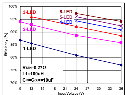
Fig 12. I_{OUT}=370mA
