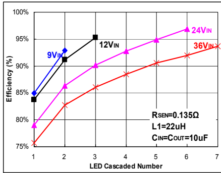
Fig 14. I_{OUT}=740mA
