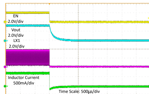
Figure 8-13. Shutdown by EN
