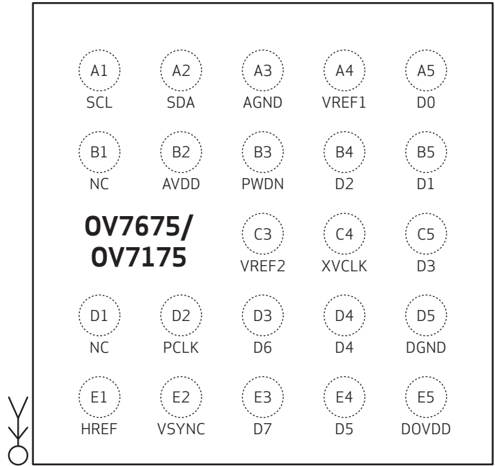
figure 1-1 pin diagram
